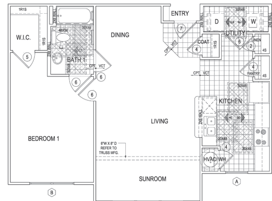
1 Bedroom Unit (A1 Plan) Alternate Plans & Handicap Accessible Plan Also Available
