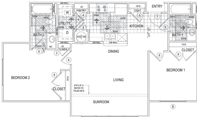
2 Bedroom Unit (B2 Plan)
